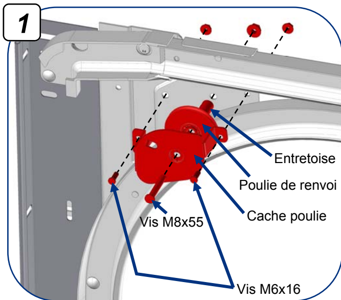
Ensemble poulie
